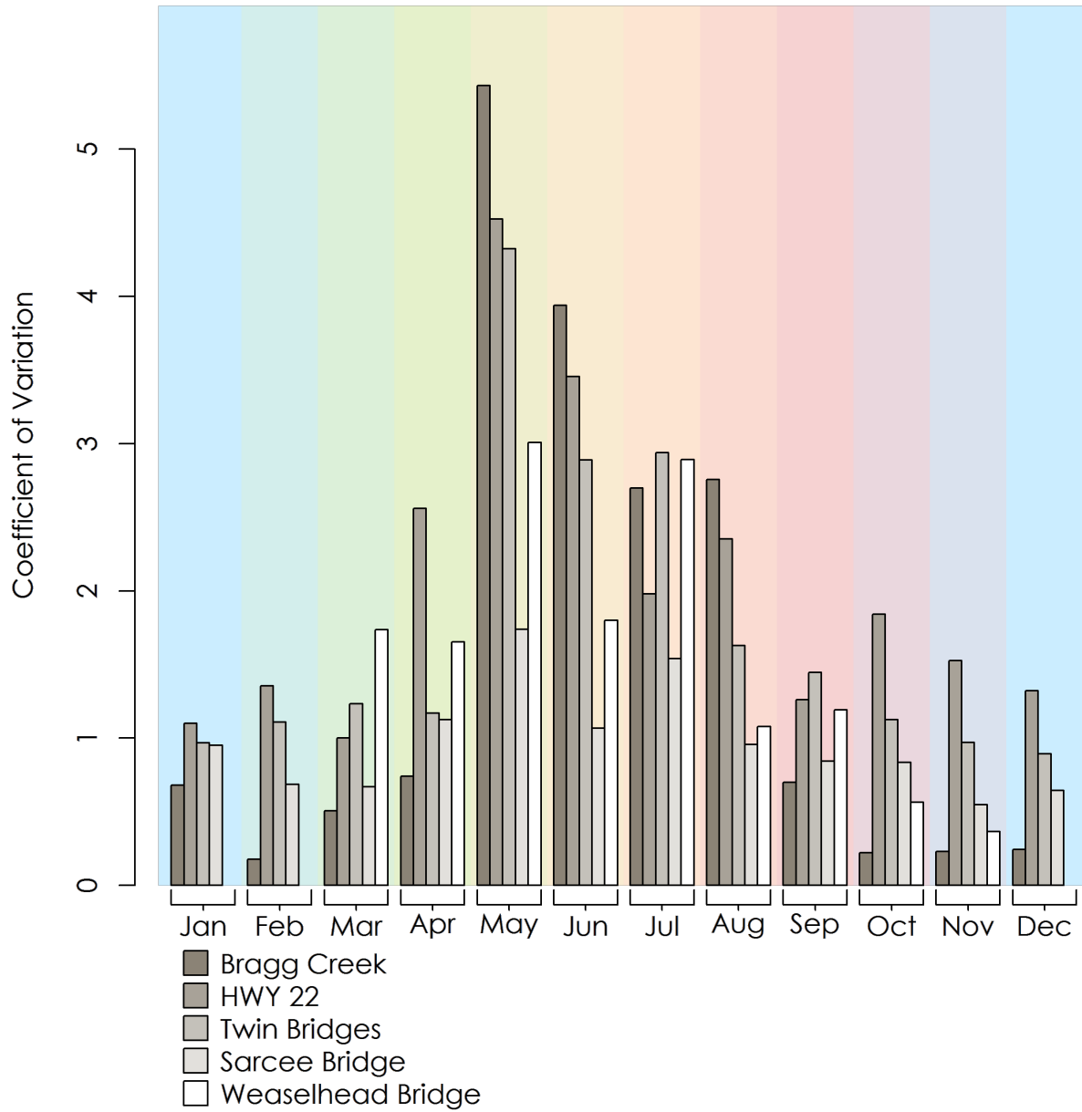
Figure 3-2 Seasonal Variation Metrics of Total Suspended Sediment in the Elbow River Mainstem and at the Glenmore Reservoir from 1979 to 2016
